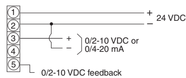
KA-175-P - KA-301-P Proportional Control 24 VDC Power 0/2-10 VDC or 0/4-20 mA Signal
